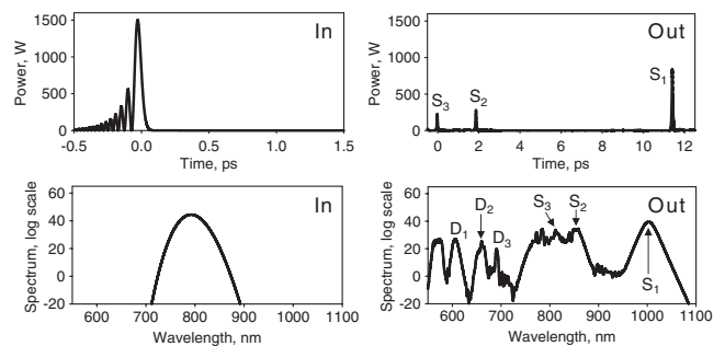
FIG. 3. Top row: Input and output temporal waveforms for an Airy pulse with -60\,000 \text{ fs}^3 cubic spectral phase propagating in a 1 m long nonlinear fiber with the parameters described in the text. Bottom row: Corresponding spectra. Solitons and dispersive waves are marked with letters S_i and D_i , where the subscript indicates their order of appearance.
