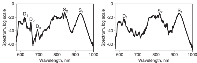
FIG. 6. Supercontinuum spectra recorded at the output of a 1 m long microstructured fiber with the parameters closely matching those used in the simulations. The case with the input Airy pulse with a negative cubic spectral phase equal -60\,000\text{ fs}^3 (left) results in the generation of three distinct dispersive-wave features. The case with the same but opposite spectral phase (right) results in the generation of only one distinct dispersive wave.
