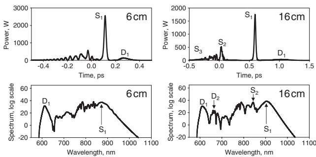
FIG. 4. Top row, left: Airy pulse with -60\,000 \text{ fs}^3 cubic spectral phase after 6 cm propagation in the fiber. The main peak of the Airy waveform has produced a soliton-dispersive-wave pair and is nearly regenerated. Right: Same after 16 cm propagation. The regenerated main peak of the pulse has produced another soliton-dispersive-wave pair. Bottom row: Corresponding spectra.
