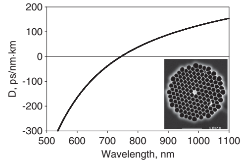
FIG. 2. Fiber dispersion as a function of wavelength. The inset shows a scanning electron micrograph of the guiding region of the fiber provided by the fiber manufacturer.
