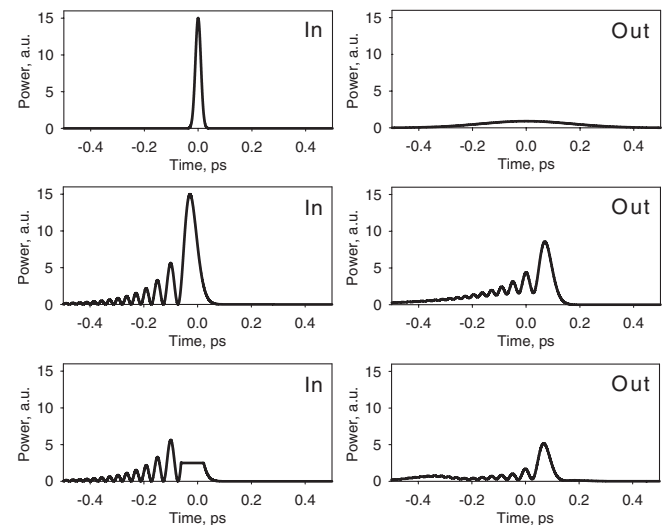
FIG. 1. Top row: Simulation of a Gaussian pulse propagating in a linear medium that has a second-order dispersion only shows a severe pulse spreading on propagation. Middle row: The input pulse is an exponentially apodized Airy pulse with the same bandwidth as that of the Gaussian pulse above. Propagation through the same medium leaves the dominant peak of the waveform largely intact. Bottom row: The dominant intensity peak of the input Airy pulse is cutoff at a level of one-sixth of the peak value. The feature is restored on propagation through the same dispersive medium as above.
