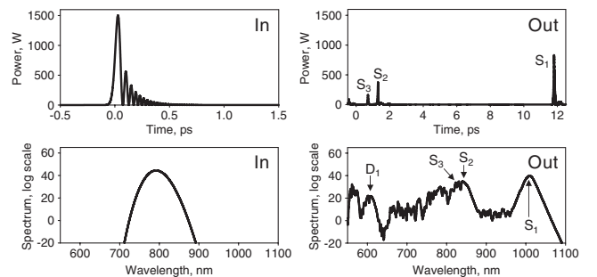
FIG. 5. Input Airy pulse with +60\,000 \text{ fs}^3 cubic spectral phase propagates in 1 m long nonlinear fiber. Top row: Temporal input and output waveforms. Bottom row: Corresponding spectra. Only one distinct dispersive-wave peak is produced.
